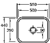
Cisterna 60C Single bowl
