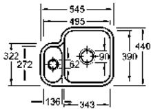
Cisterna 60B 1.5 bowl
